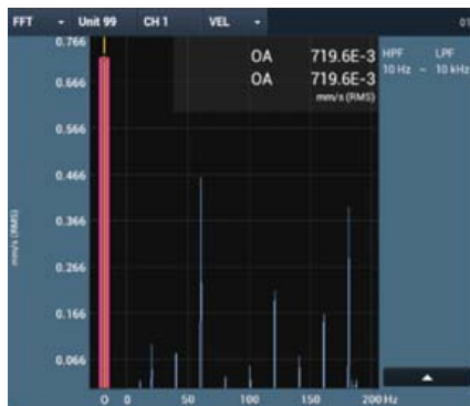
FFT spectrum
