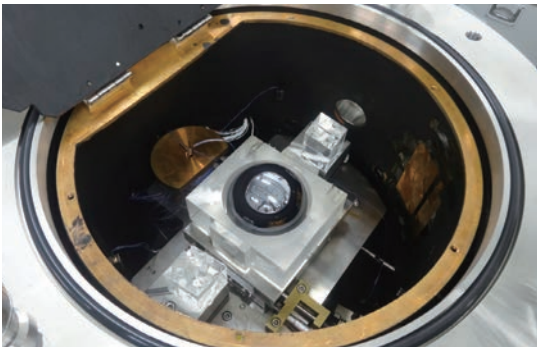
Fig.2 Instrument used to measure the diameter of a silicon sphere ©AIST
