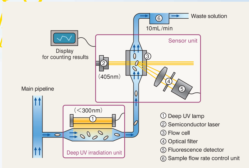
Fig. 2. Schematic diagram of bioparticle counter configuration Deep UV irradiation unit: Specifically intensifies microbe autofluorescence. Sensor unit (sensor designed to detect fluorescence only): Detects microbe autofluorescence.
